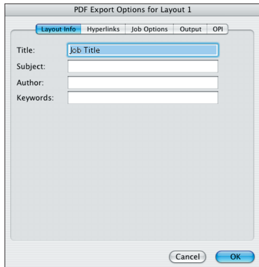
Layout Info
