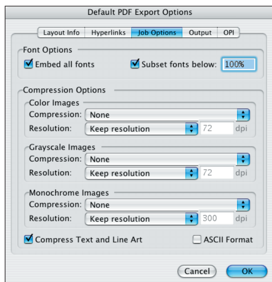
Job Options
